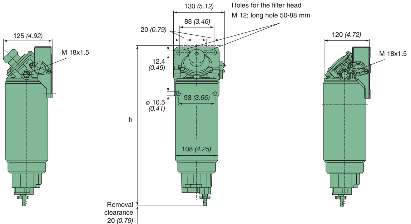
PreLine® with manual pump
