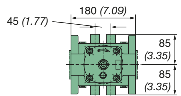
Fig. 3 Filter insert removable from above
