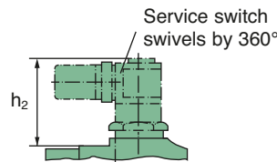
Service switch installation height
