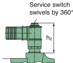
Service switch installation height
